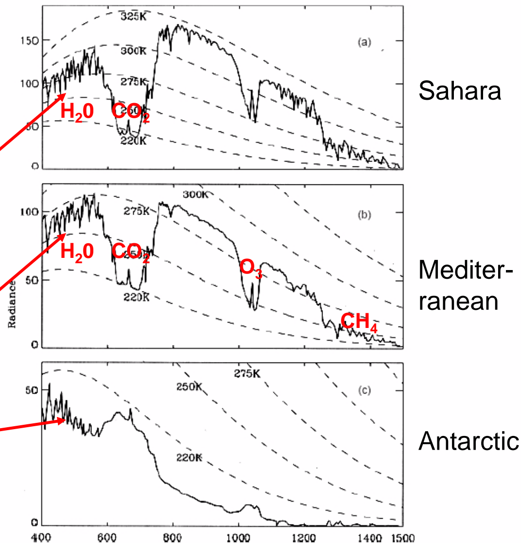
Figure 9: Emission spectra of the Earth taken by the Nimbus 4 satellite. The radiance units are milliWatts per square metre per cm -1 per steradian. Spectrum (a) is measured over the Sahara Desert, spectrum (b) over the Mediterranean, and spectrum (c) over the Antarctic
